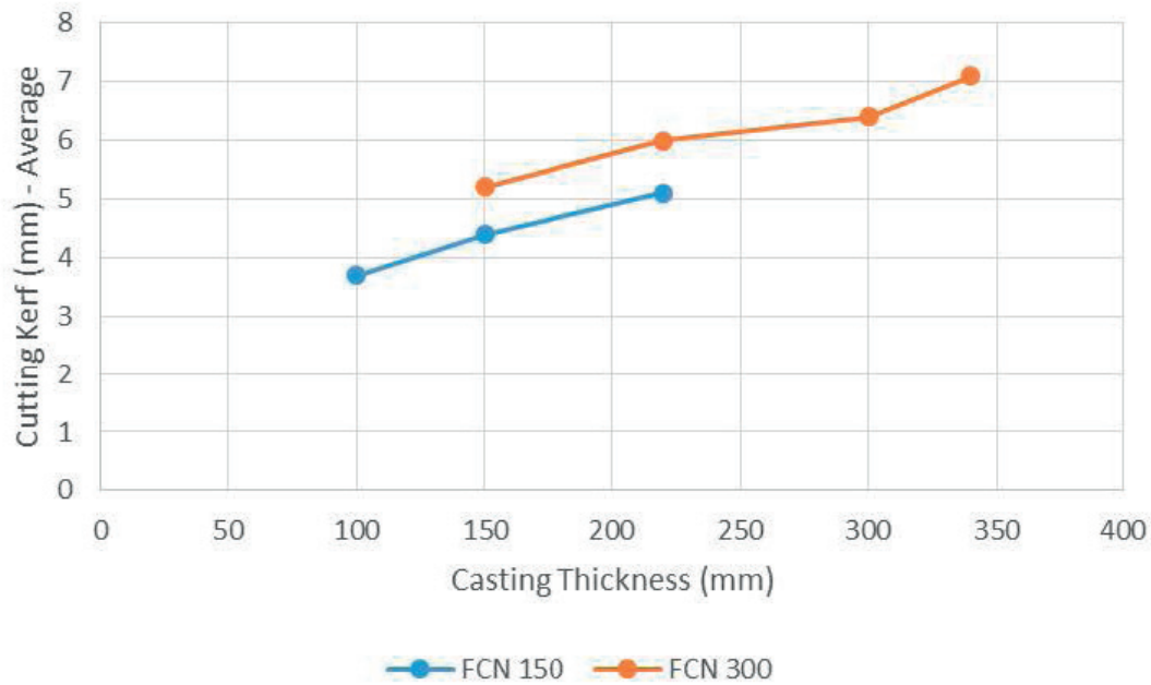
Cutting kerf in relation to material thickness
